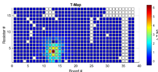
Figure 2: Example of a quench due to a surface defect captured on the T-Map.
