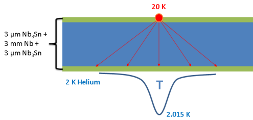
Figure 3: Diagram of a simulated point heat-source. The material has three layers – Nb_3Sn on the vacuum surface, Nb substrate, and then Nb_3Sn on the outside of the cavity.
