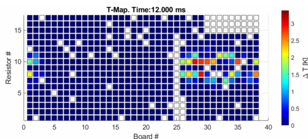
Figure 1: Example of a suspected multipactor quench captured on the T-Map.
