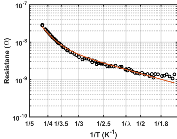
Figure 6: Measured BCS resistance vs. inverse temperature for a 1.3 GHz cavity with a typical Nb_3Sn coating scheme with a best fit line.
