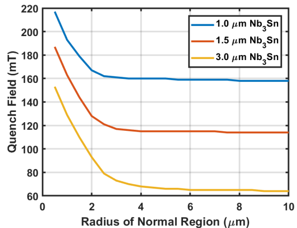
Figure 5: Quench field of various thicknesses of Nb_3Sn films on a Nb substrate vs. the radius of the normal conducting region from thermal modelling.
