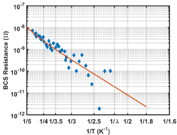
Figure 7: Measured BCS resistance vs. inverse temperature of a high tin-availability Nb_3Sn 1.3 GHz cavity with a best fit line.
