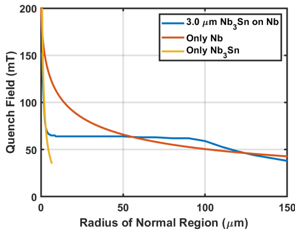
Figure 4: Quench fields of various materials as a function of the radius of the normal conducting region from thermal modelling.
