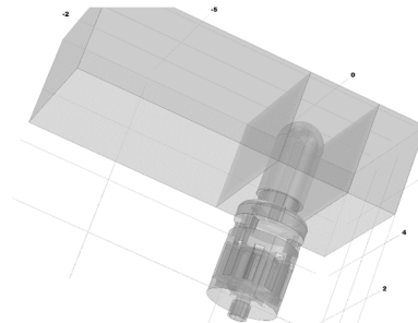
Figure 6: COMSOL Model of Tube and Launcher.
