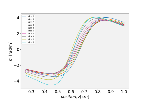
Figure 2: Evolution of the TPS slope m (Eq. (7)) as a function of the position in the drift. Each color represents one of the 10 slices the bunch has been divided into, where slice number 0 and 9 represents respectively the tail and the head slice.
