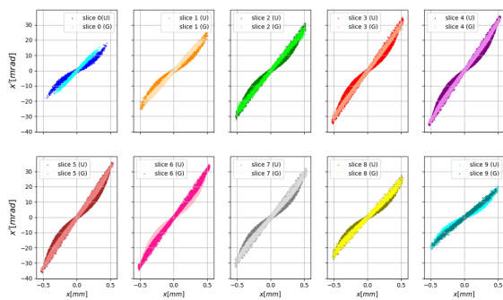
Figure 3: Slices comparison in the TPS for the beam just generated by the cathode. The two different colors in each plot represent the Cut-Gaussian and Flat-top distributions respectively, for each of the 10 slices.
