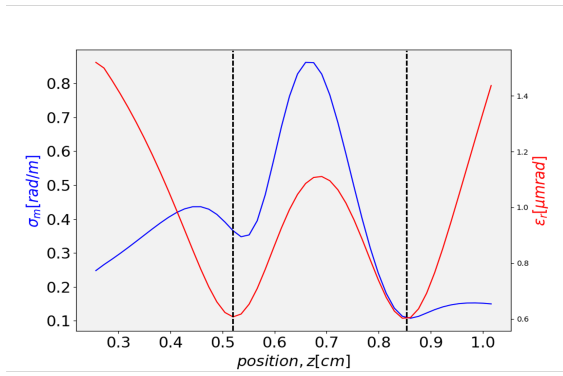
Figure 1: The slope spread \sigma_m of the TPS (blue curve) as a function of the drift position, in comparison with the rms emittance oscillation (red curve). The two vertical black dotted lines represent the exact position of the two emittance minima.
