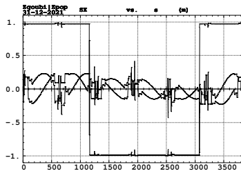
Figure 11: \vec{n}_0 components around RHIC Blue. 255 GeV.
