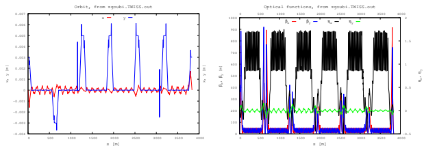
Figure 8: Blue orbit (left) and optics (right) at injection.
