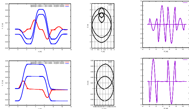
Figure 4: Top row: Helical orbit through the R+R-R+R-series, before and after helix centering in the snake. Left: Y(s) , Z(s) ; middle: (Y,Z) projected helix; right: field B_Z(s) , largely independent of possible mis-centering of the helix. Bottom row: same, for the R+0R-0 series at 300 A.
