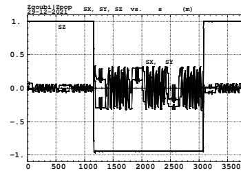
Figure 7: Components of the periodic spin vector around RHIC Blue. Origin s=0 is at STAR.
