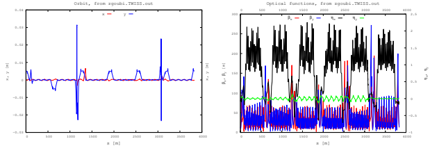
Figure 5: Blue orbit (left) and optics (right) at injection. The 9 and 3 o'clock local snake bumps are apparent, to the left of respectively the IP8 and IP4 vertical separation bumps.
