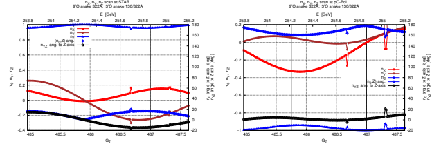
Figure 12: G\gamma scans of \vec{n}_0 components and angle to Z-axis at STAR (left) and pC-polarimeter (right). \vec{n}_{YZ} is the projection of \vec{n}_0 in the (Y,Z) plane, a quantity measured at pC-polarimeter.
