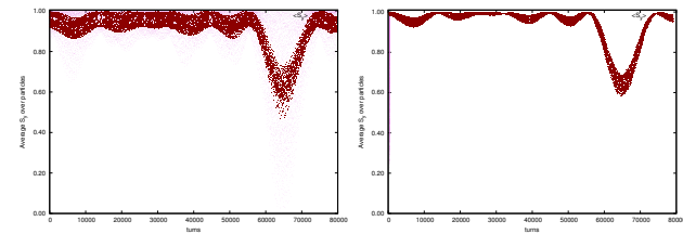
Figure 13: Crossing of 393 + z, with 9 O'clock snake 88% (left) or 100% (right). Red curve: \langle S_Z \rangle (turn) average over 3 particles; blue: the 3 individual motions.
