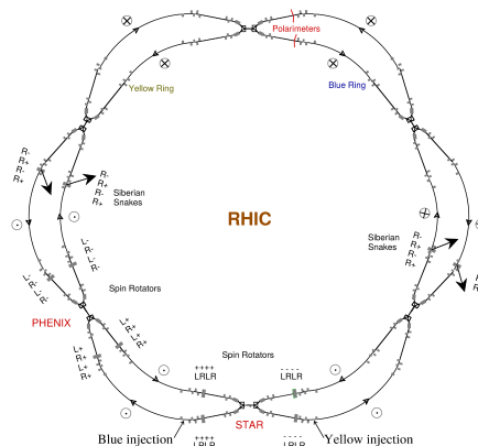
Figure 2: Location of snake series R+R-R+R- and R-R+R-R+ in Blue and Yellow rings, at 9 o'clock and 3 o'clock. Beam goes clockwise in Blue, counter-clockwise in Yellow.
