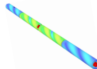
Figure 3: OPERA model of RHIC four helical module snake.
