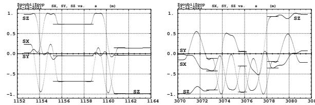
Figure 10: Spin \vec{n}_0 components across 9 (left) and 3 o'clock (right) snake, at 255 GeV.
