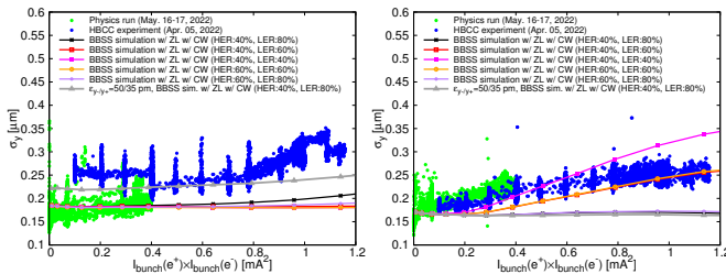
Figure 4: Vertical beam sizes of electron (left) and positron (right) beams at the IP predicted by BBSS simulations compared with experiments.
