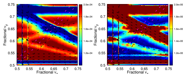
Figure 2: Tune scan of luminosity (left) and vertical beam size (normalized by \sigma_{y0} ) for the parameter set of 2019.07.01 with the LER as the weak beam in the BBWS simulation. Important resonant lines are plotted, and the black dot indicating the working point for machine operation.
