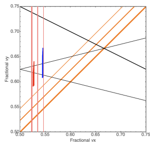
Figure 1: Beam-beam driven footprint of LER beam in the tune space with parameters of Table 1. The blue and red footprints represent 2019.07.01 and 2022.04.05, respectively.
