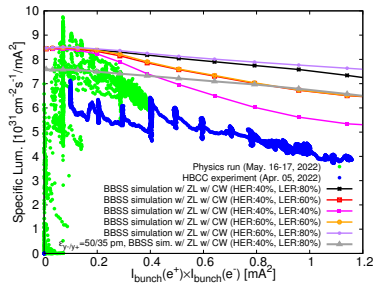
Figure 3: L_{sp} predicted by BBSS simulations with inclusion of longitudinal impedances and from experiments of high-bunch current collision (HBCC) machine study and physics run.
