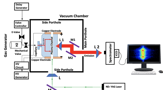
Figure 1: Scheme of the experimental set-up used at the SPARC_LAB test-facility to form and characterize plasma in a gas-filled capillary. An optical path is designed for guiding the plasma light into the spectrometer. L1, L2, represent lenses and M1, M2 indicate mirrors. The Copper electrodes have mounted on the capillary extremities. An Nd: YAG laser probe of 532 nm is used for the optical alignment.
