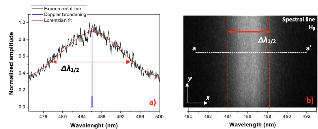
Figure 2: Balmer beta line measurements: a) transverse profile of the Balmer beta line corresponding to the cut aa' with the overlapped Lorentzian fit (Stark effect) and the contribution of the Doppler effect calculated for a plasma temperature of 2 eV, and b) image of the spectral line acquired via the ICCD camera.
