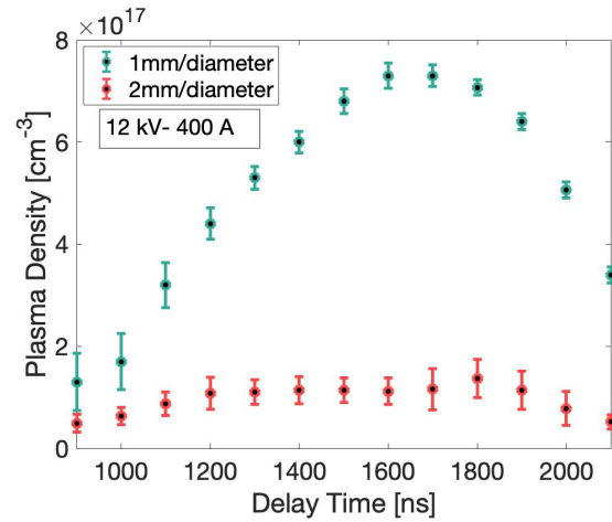
Figure 3: The variation of averaged electron density as a function of delay time after the discharge trigger in the targeted capillaries of 3 cm/long-1 mm/diameter and 3 cm/long-2 mm/diameter with a double-inlet system. The reported error bars represent the standard deviation calculated by 50 independent plasma density profiles (in a duration of 100 ns gate width).
