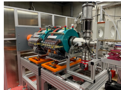
Figure 4: Test stand for the main electron components and diagnostics at Goethe-University Frankfurt.
