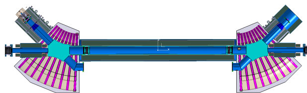
Figure 1: Preliminary 3D model of the SCC electron lens.
