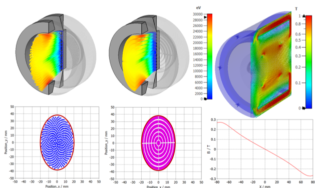
Figure 5: Simulated beam extraction for a beamlet-style grid (left), a target-style grid (middle) and magnetic system including a quadrupole for beam shaping with corresponding B_x (right).
