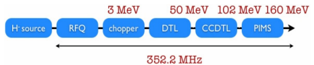
Figure 4: Linac4 layout.
