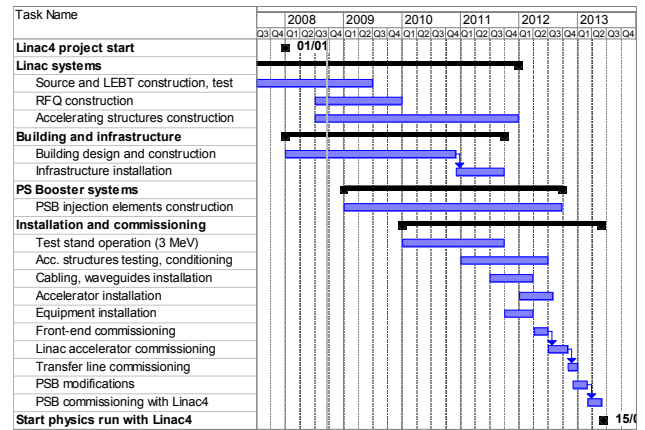
Figure 7: Linac4 Masterplan.
