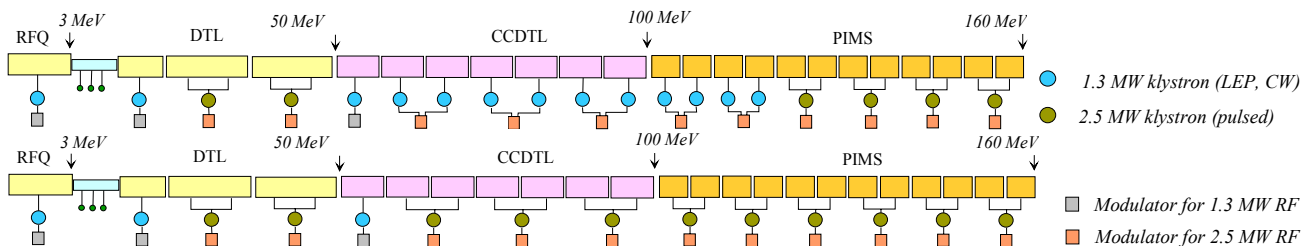
Figure 5: RF power distribution at installation (top) and after the end of the stock of LEP klystrons (bottom).
