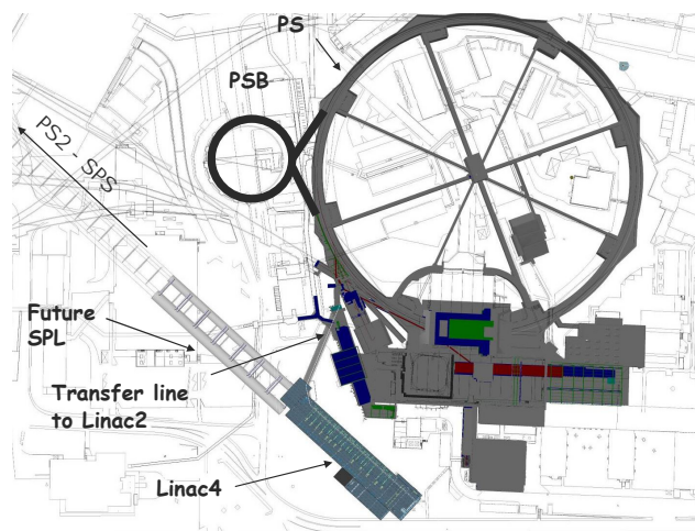
Figure 2: View of the PS Complex at CERN, showing the position of the new Linac4.
