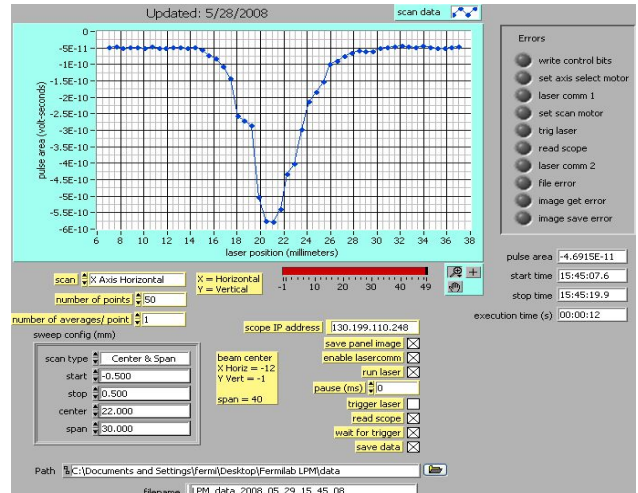
Figure 4: The Labview page showing a profile measurement.
