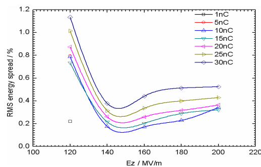
Fig. 6: RMS energy spread dependence on the photocathode peak electric field and bunch charge.
