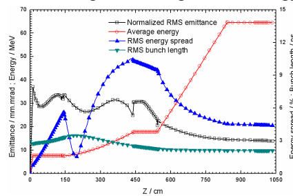
Fig. 11: Emittance, energy, energy spread and bunch length variation along the injector (20 nC, 160 MV/m).
