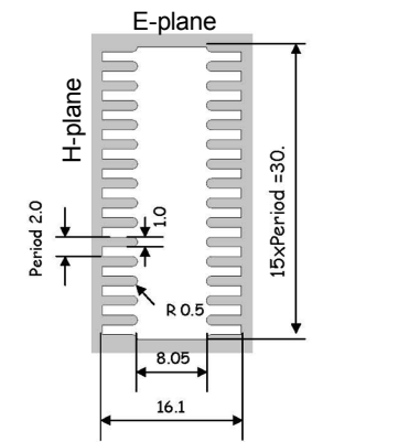
Cut - off frequency = (11.424 -0.09) GHz Losses at 11.424 (SS430: \sigma=1/52 \text{ Cu} , \mu=6 ) = 50 dB/m
