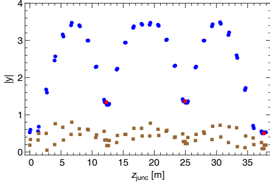
Figure 4: For f = 4 GHz: the quantity |y| for right going waves (blue) and left going waves (brown); |r_{n,1}| for absorbers is shown in red. For this case p_{2K}/p_{tot} = 0.17 .
