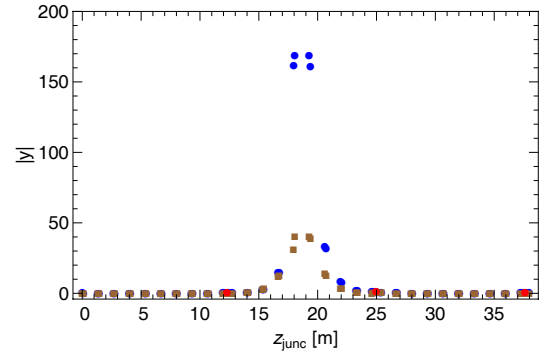
Figure 6: For f = 16 GHz and \Delta z = 0.8 mm: |y| for right (blue) and left (brown) going waves in the first mode ( m = 1 ); |r_{n,1}| for absorbers is in red; p_{2K}/p_{tot} = 0.95 .
