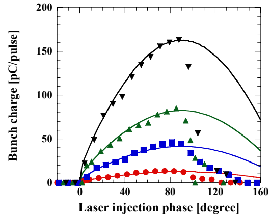
Figure 2: Bunch charge as a function of laser injection phase. The plots indicate laser power of 3, 10, 20, and 40 \mu\text{J}/\text{pulse} from the lower. The lines are simulation results according to Eq. (1).
