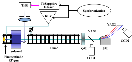
Figure 1: Schematic diagram of femtosecond electron gun measurement.
