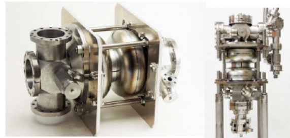
Figure 1: 2-cell cavity #2 (five HOM couplers).
