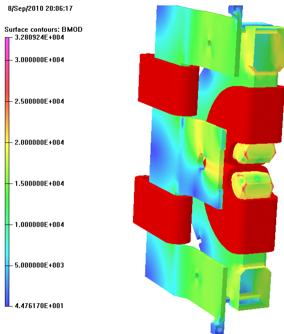
Figure 3: Cut view of the 3D model with a quad and steering magnets.
