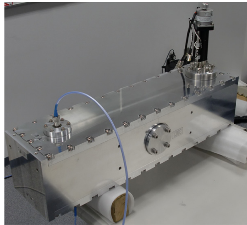
Figure 6: New buncher.
