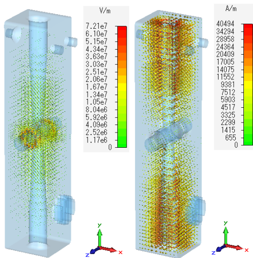
Figure 5: RF simulation. Left: electric field, Right: magnetic field.
