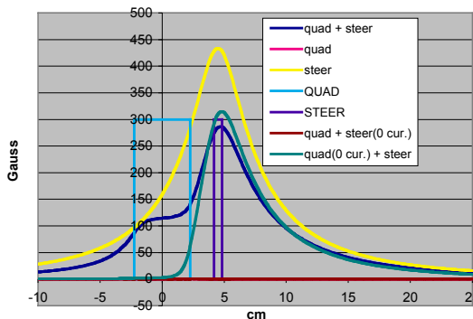
Figure 4: Cross talk of steering field.
