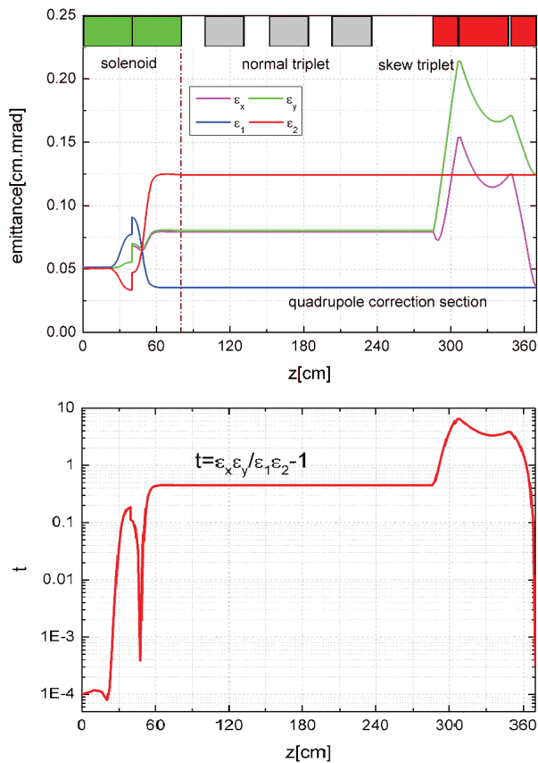
Figure 5: The emittances and the beam rms sizes along the longitudinal field and quadrupole correction section.
