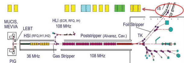
Figure 1: Conceptual layout of the transverse emittance transfer section in the GSI UNILAC.
