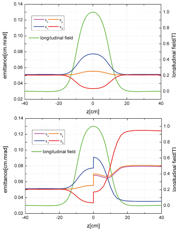
Figure 3: The rms-emittances and eigen-emittances along the longitudinal field without and with stripper foil.
