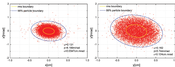
Figure 6: The particle distributions at the end of beam line.
