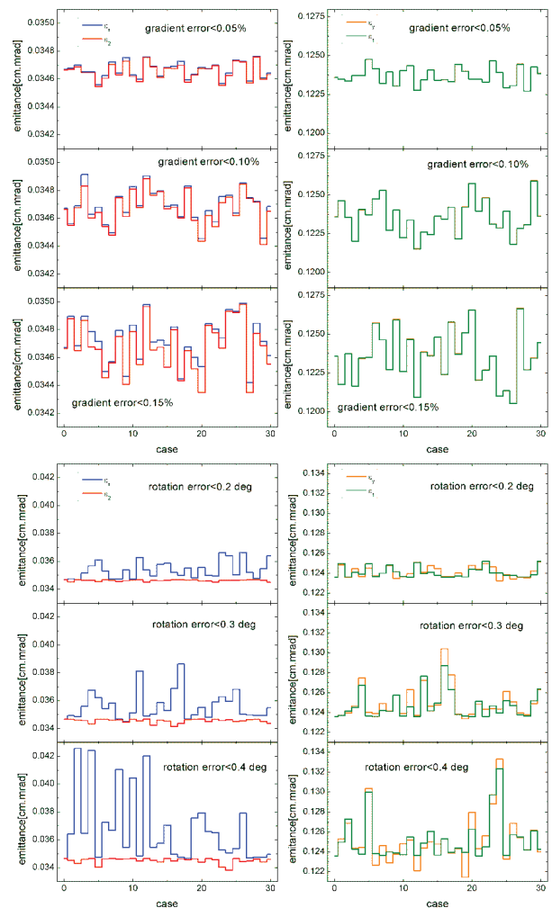
Figure 7: The influences of the gradient fluctuation and rotational angle errors.
