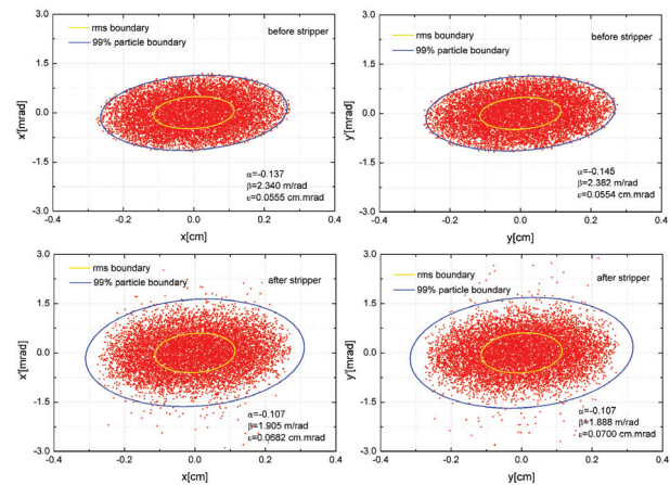
Figure 4: The particle distributions before and after foil.
