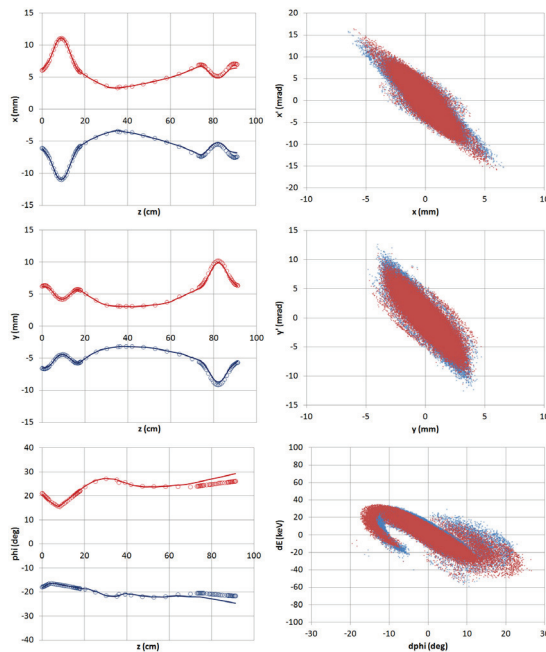
Figure 6: Beam envelopes (L) with circles by Lorasz and curves by TraceWin and output particle distributions (R) with blue dots by Lorasz and red dots by TraceWin.
