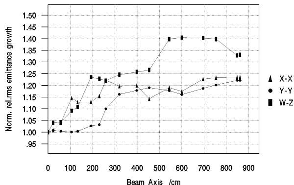
Figure 10: Emittance evolutions along the CH-DTL.
