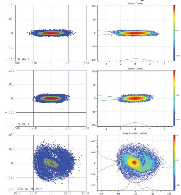
Figure 3: RFQ output particle distributions given by the ParmteqM (L) and Toutatis (R) codes.
