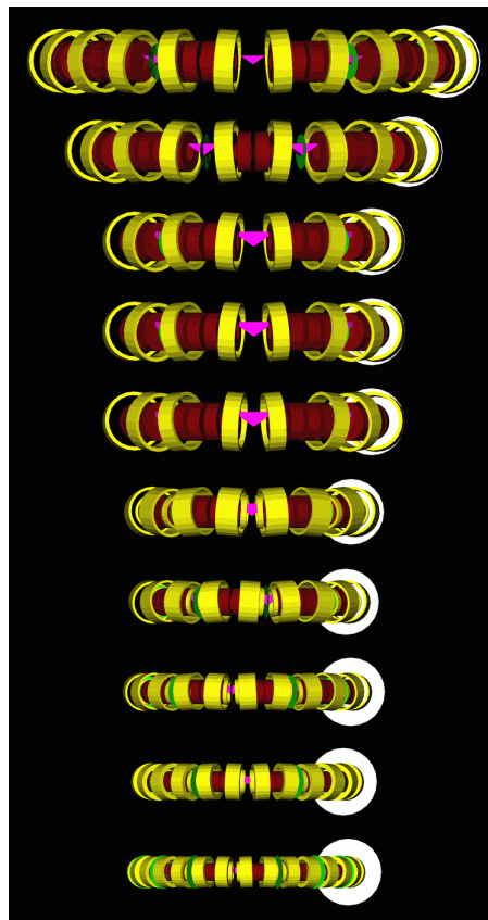
Figure 3: Geometry of the first 10 stages of the tapered Guggenheim.
