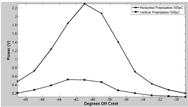
Figure 3: Experiment: For CSR, the horizontally polarized component has approximately 5 times more power than the vertical one. The charge was 500 pc and the number of bunches was 40.
