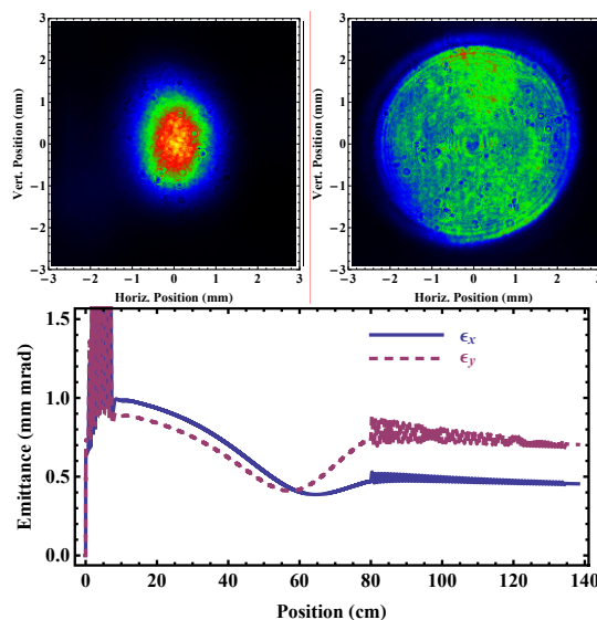
Figure 2: Top: Profiles before and after refractive beam shaper. Left: before, Right: after. Bottom: Simulated emittance growth of electron beam through X-band gun and first accelerating section with starting distribution shown above
