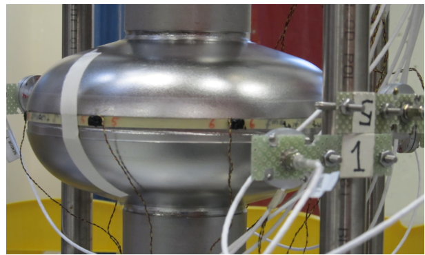
Figure 1: OSTs installed on 1-cell cavity.
