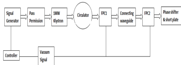
Figure 3: BNL FPC conditioning block diagram.
