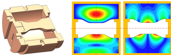
Figure 1: Cross-section of the dual-moded cavity (left) and the electric (top half) and magnetic (bottom half) fields of the TE_{011} (middle) and TEM_3 (right) modes that couple in from the left and right side, respectively.
