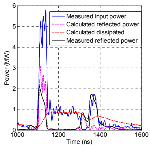
Figure 6: Comparison of the (a) TE 011 and (b) TEM 3 measured and computed reflected power. Also shown are the input power and computed dissipated power.
