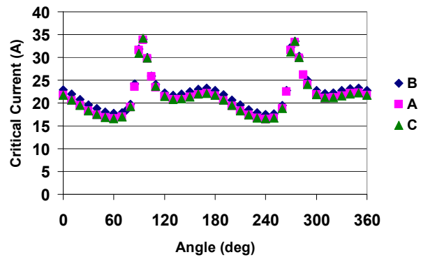
Figure 5: Critical Current at different sections at the same magnetic field (0.5 T) at a low dose level (2.5 \mu A -hr) for SuperPower samples.
