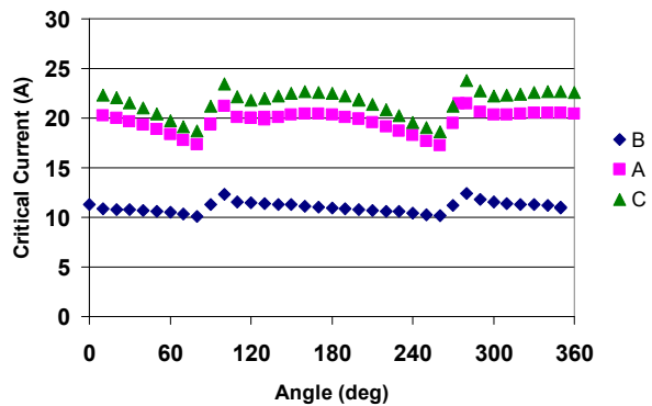
Figure 6: Critical current at three different sections at 0.5T at a high dose level (100 \mu A -hr) for SuperPower samples
