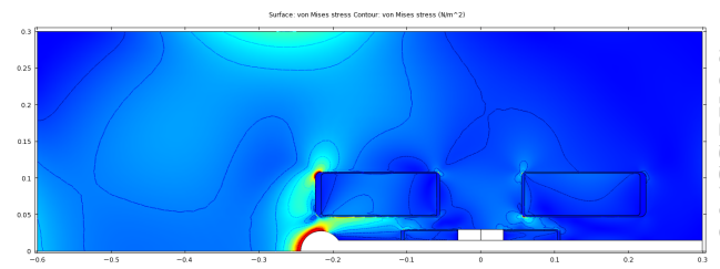
Figure 6: Von Mises stress in structure of “C” shape, w/o the right-hand absorber, to eliminate its backscattering of radiation; maximum \sigma_{vM} to left of keyhole = 353 MPa.
