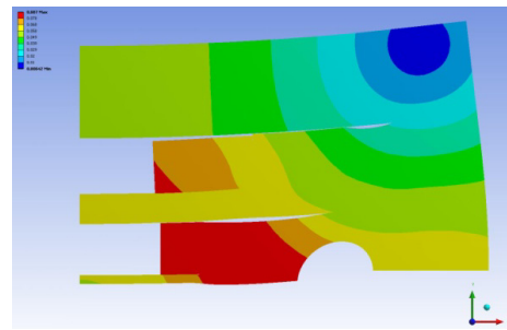
Figure 10: Total deformation \delta on support structure at B_0 = 10.7 T; \delta_{\max} = 87 \mu ; coil \delta_{\max} \approx 20 \mu .
