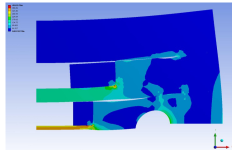
Figure 9: Von Mises stress, \sigma_{vM} , at B_0 = 10.7 T, which overestimates the stress by 21%; max. \sigma_{vM} \approx 400 MPa.
