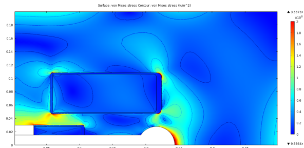
Figure 3: Contours of von Mises stress, \sigma_{vM} . The maximum value to the right of the keyhole is 246 MPa at 10 T; the average tension in the web is ~150 MPa.
