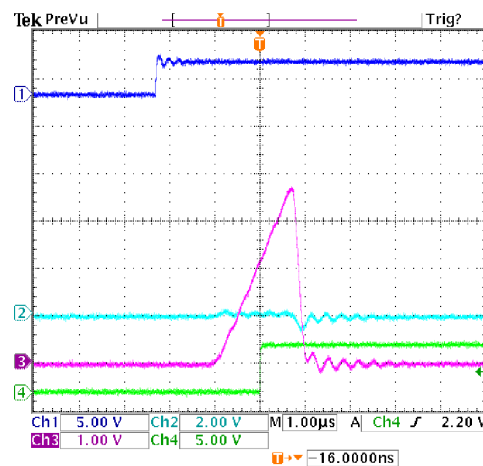
Figure 5: Scope trace shows shorting the cathode to ground through a length of #40 AWG wire. DTI's rapid fault detection and current limiting circuitry, leaves the wire intact. Switch opening occurs approximately 700 ns after the threshold current limit is reached, and the peak current remains below ~150 A.
