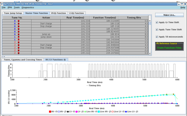
Figure 6: Timing function display, with HV capacitor charging shown as a level 4 and magnet pulse as an 8.
