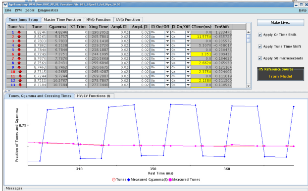
Figure 5: A detail of the display of fraction remainder of G-gamma and Horizontal Tune.
