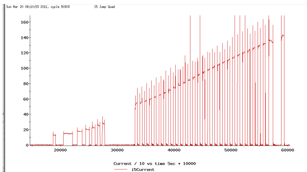
Figure 3: Current vs. time in an AGS cycle, the gap is around transition where the beam is less well behaved. The first and last pulses as they only jump one resonance. The early and late pulses are longer due to lower gamma dot.
