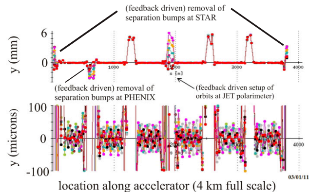
Figure 9: Orbit measurements as beams are brought into collision by removal of the vertical separation bumps.
