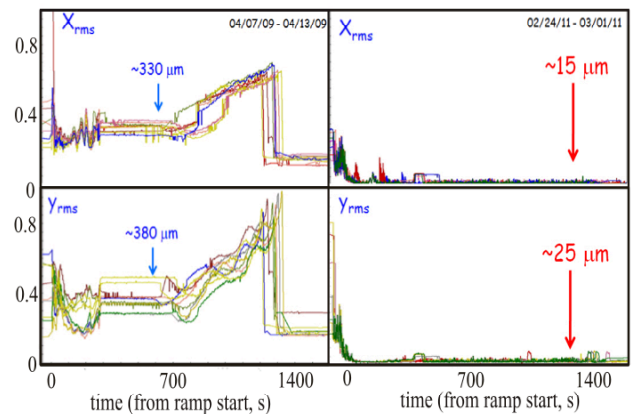
Figure 6: Superposition of measurements from multiple ramps of horizontal (x) and vertical (y) orbit rms measured without (left, run-09) and with (right, run-11) orbit feedback.
