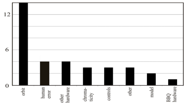
Figure 4: Histogram of ramp failures during 14 different commissioning periods of run-09.
