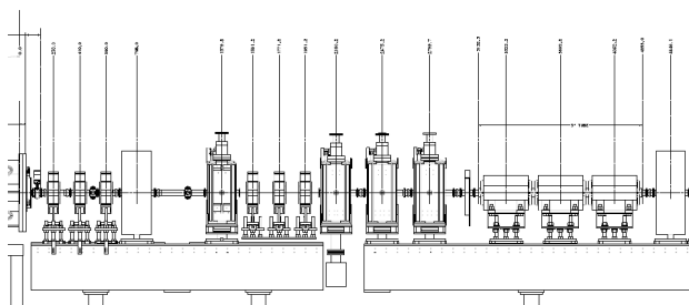
Figure 4: The acceleration section of the six cavity test. The first item after RFQ is a quad triplet, followed by a buncher cavity and spoke resonator. These are followed by a quad triplet, spoke resonator triplet, quad triplet combination. The final item before the diagnostic line is a buncher cavity.
