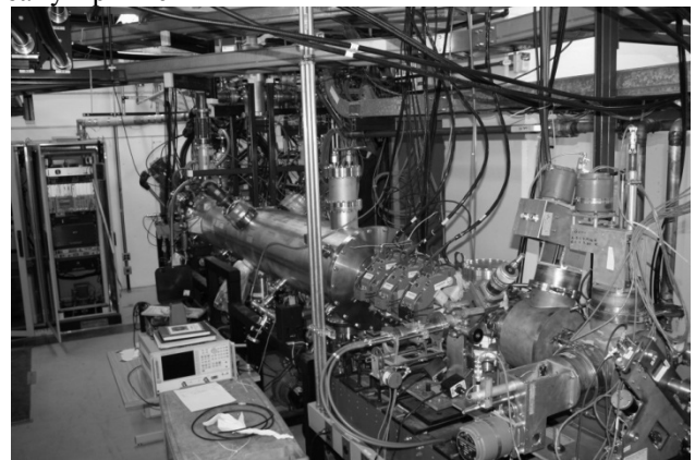
Figure 2: Front of 2.5 MeV beam line showing ion source, RFQ, quadrupoles, longitudinal profile monitor, fast Faraday cup, and wire scanner.
