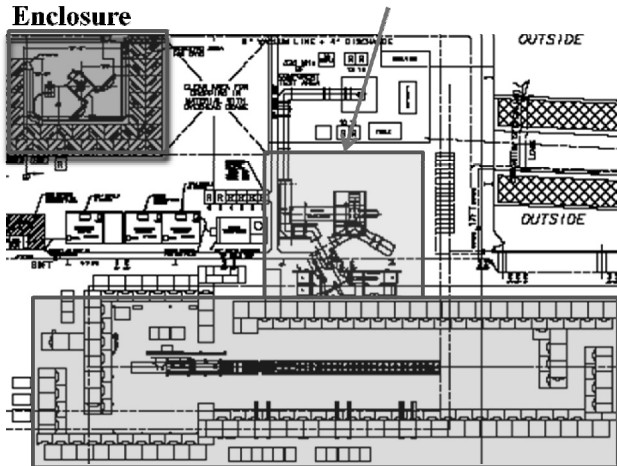
Figure 1: Layout of the Project X front-end test facility.
