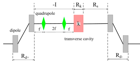
Figure 2: A chicane-type exact EEX beam line.
