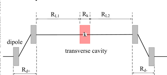
Figure 1: Cornacchia-Emma's EEX beam line.
