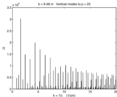
Figure 1: \text{Re}Z(n, n\omega_0) in ohms vs. k = n/(2\pi R) in \text{cm}^{-1} for VUV parameters
