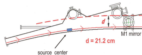
Figure 7: Flared vacuum chamber at IR ports of CLS.
