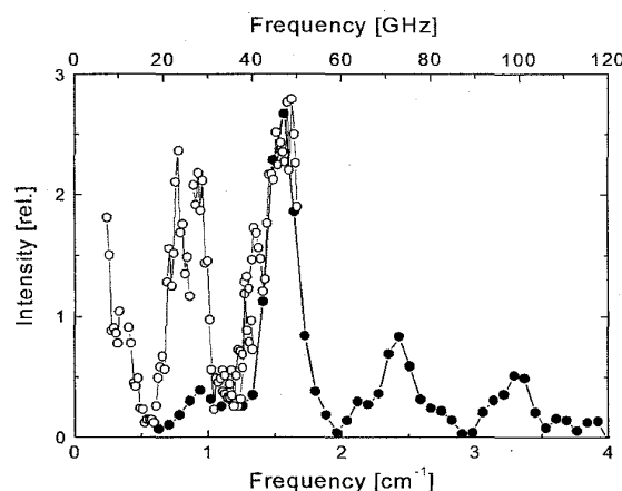
Figure 3: Long wavelength spectrum measured at NSLS VUV.
