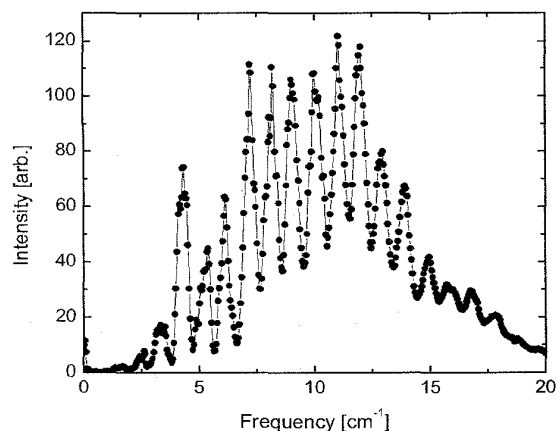
Figure 2: Far IR spectrum from interferometer at NSLS VUV.
