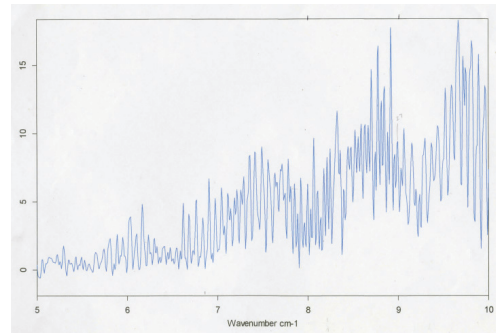
Figure 5: Typical CSR spectrum at CLS.
