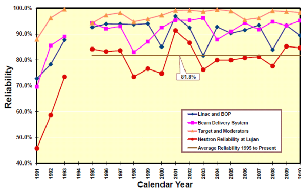
Figure 2: Sub-system reliability for beam delivery to the Lujan Center
