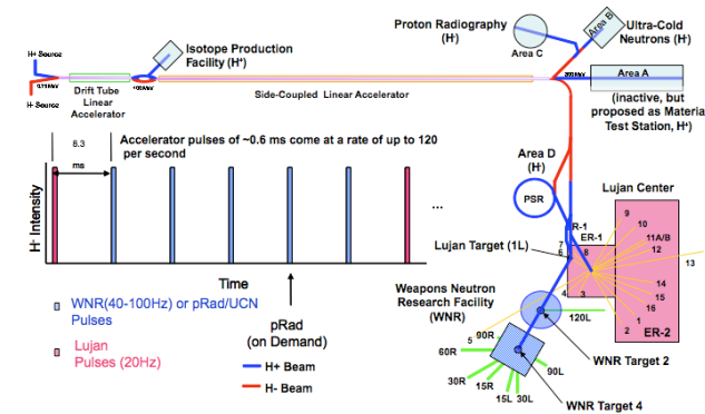
Figure 1: Schematic layout of the LANSCE User Facility
