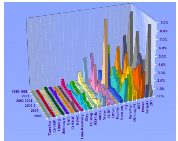
Figure 4: Historical sub-system down time for beam delivery to the Lujan Center
