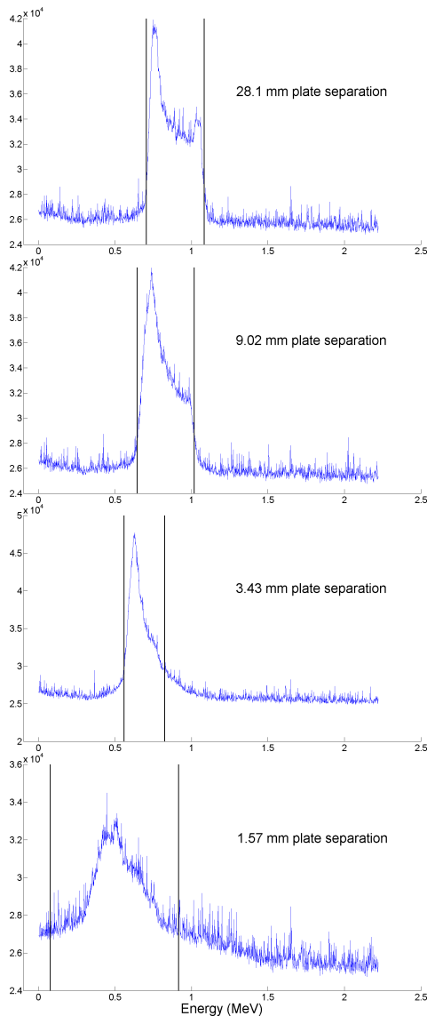
Figure 5: Energy spectrum plots at various plate separations. Note that closing the gap too much (smaller than ~3.4 mm) results in a larger energy spread. The vertical lines designate the width where the intensity falls to 20% of the maximum height over the background.
