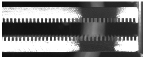
Figure 4: Side view of corrugated plates. Beam travels left to right. Note the corrugations are longitudinally misaligned by about a quarter of a period.
