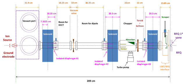
Figure 1: PXIE LEPT layout schematic.
