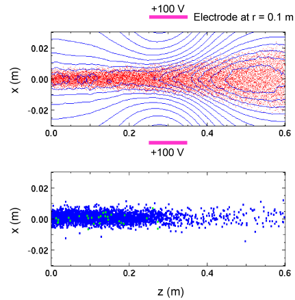
Figure 2: WARP 3D simulation of the transition from neutralized to un-neutralized transports in the PXIE LEBT. Electrode keeps positive ions (blue dots) from drifting into the un-neutralized region. For the un-neutralized region, we assume the vacuum is so good that there is little ionization processes. Note that most electrons (green dots) are expelled.
