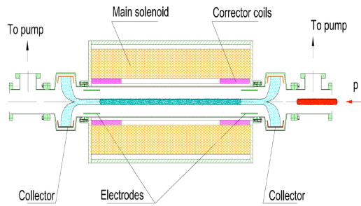
Figure 3: A conceptual layout of the electron-column apparatus for space-charge compensation in the IOTA ring.
