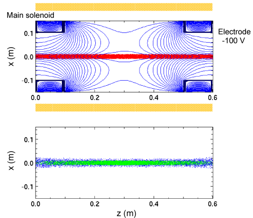
Figure 4: WARP 3D simulation of the plasma formation and trapping in the e-column. A uniform solenoid keeps both electrons (green dots) and ions (blue dots) in the beam path. Ions are slowly escaping longitudinally. To resolve cyclotron motion of the electron, the time step has been set to \Delta t \leq 0.25 \times 2\pi/\omega_{ce} .
