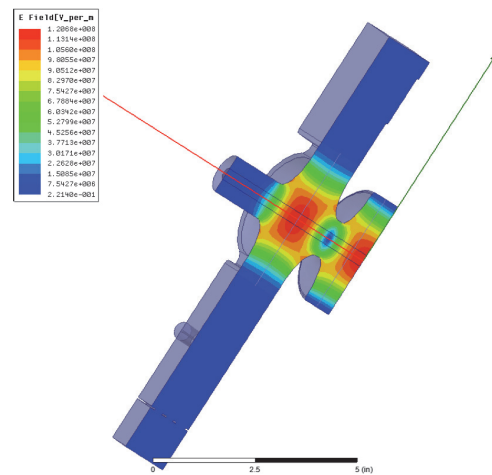
Figure 1: 3D model used for HFSS simulation. Surface electric field is shown.
