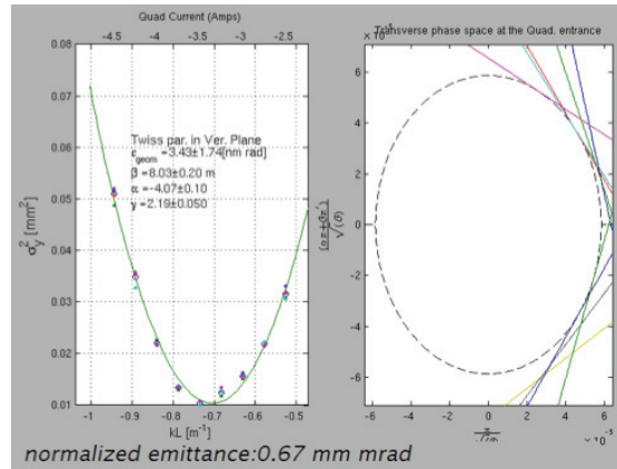
Figure 9: Initial emittance measurement of a 500pC beam.
