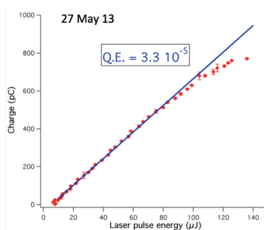
Figure 8: Charge yield as function of laser energy.
