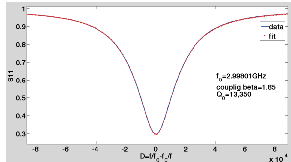
Figure 3: Reflection coefficient. Data (red dots) and fit (blue line).
