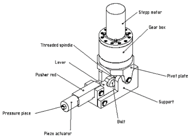
Figure 4: Drawing of tuner foreseen in the superconducting half wave resonator module.
