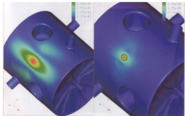
Figure 7: Deflection of the outer niobium housing due to a point load calculated using ProEngineer. The resulting tuning sensitivity is 14 Hz/micron of deflection.
