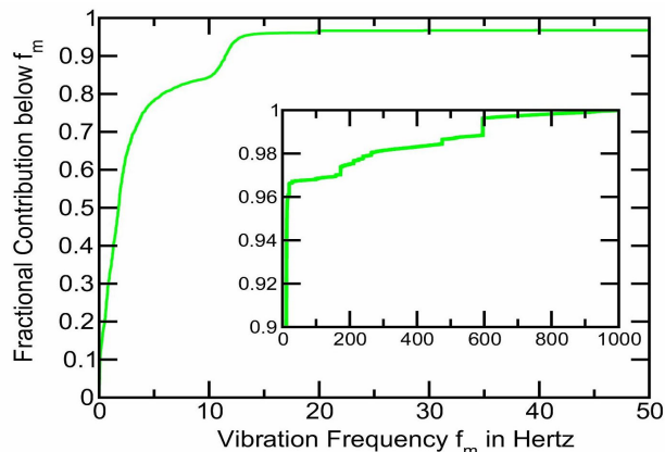
Figure 4: Fractional contribution below the frequency f_m . The inset shows the same curve extended to vibrational frequencies up to 1 kHz.
