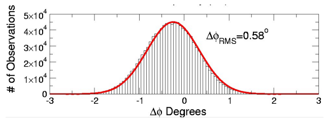
Figure 6: Phase error distribution for the two-spoke cavity at E_{\text{ACC}}=6.5 MV/m locked in both phase and amplitude to an external master oscillator.
