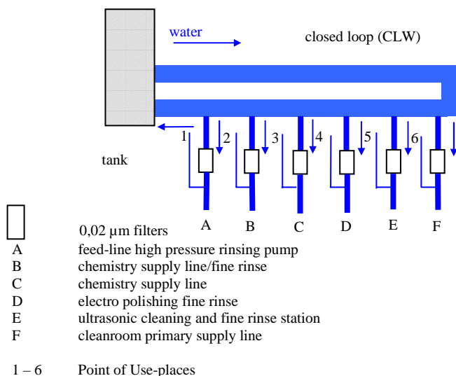
Figure 6: UPW-circulation
