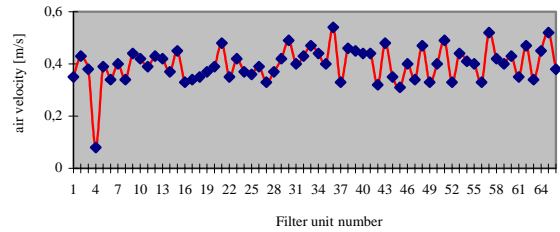
Figure 4: Air velocity distribution of the TTF cleanroom with broken butterfly valve on filter unit Nr. 4
