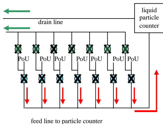
Figure 7: Schematics of the UPW switchboard connection to the inline liquid particle counter
