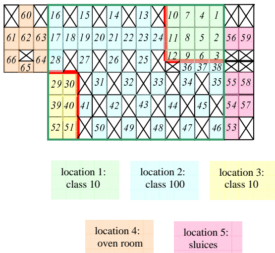
Figure 3: Filter unit number and location of all absolute filters in the TTF cleanroom
