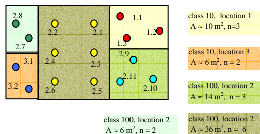
Figure 1: Location and number of measurement points at the TTF class 10 / 100 area
