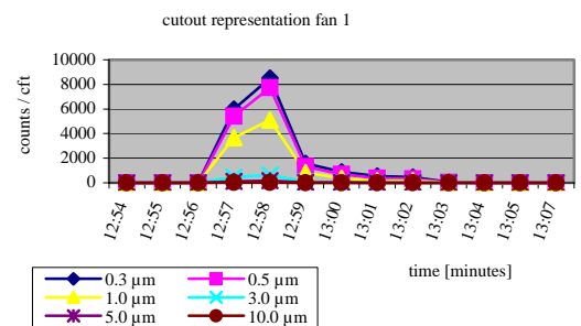
Figure 5: Typical cleanroom recovery time after shut down of the fan units (fan is working again at 12:56)
