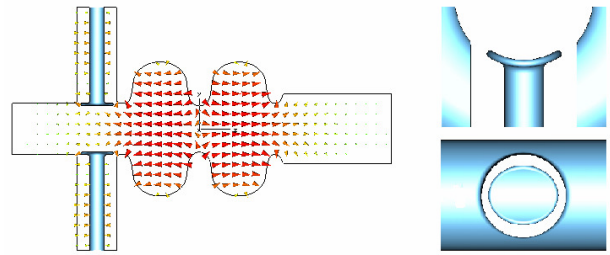
Figure 38: Two-cell cavity with the twin-coaxial input coupler and details of the coupler-cavity interface [50].
