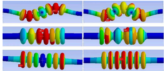
Figure 36: Example of vibration modes of a 7-cell cavity: transverse, longitudinal, breathing (ANSYS simulations). (Courtesy of M. Liepe, Cornell University.)
