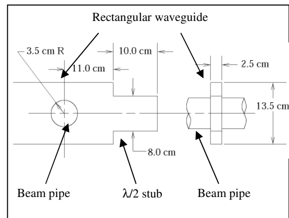
Figure 34: The cavity/coupler interface of the original CEBAF cavities [9].
