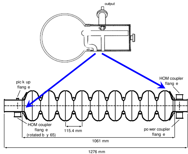
Figure 27: Coaxial loop coupler for superconducting TESLA cavities [17].
