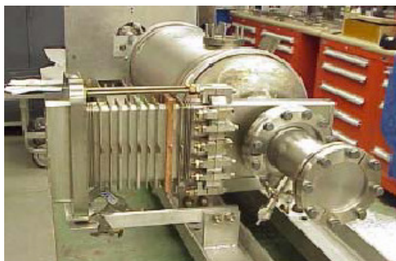
Figure 31: Waveguide coupler for CEBAF upgrade cryomodule [42].
