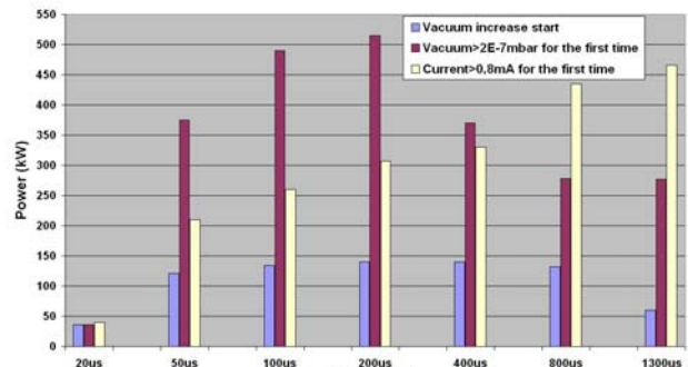
Figure 5: Lowest power levels corresponding to the first attainment of some arbitrary event levels (study done on 6 coupler pairs).
