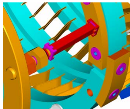
Figure 4: supports for the fixing of fast elements
