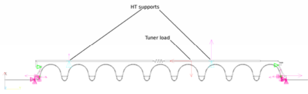
Figure 6: FE model for the analysis of displacements
