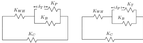
Figure 5: Equivalent spring models
