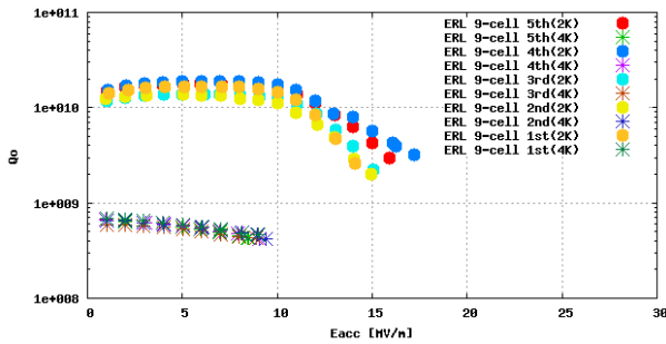
Figure 9 : Results of vertical tests for KEK-ERL model-2 cavity.
