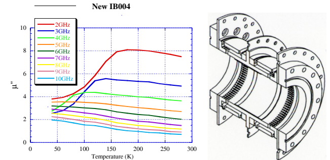
Figure 16: (Left) Temperature dependence of ferrite IB004. (Right) Schematic view of the HOM absorber.
