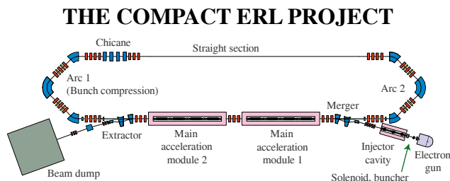
Figure 1: Conceptual layout of the Compact ERL.
