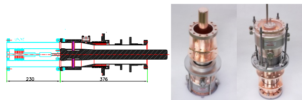
Figure 5: (Left) Design of the input coupler. (Right) Proto-type of input coupler.
