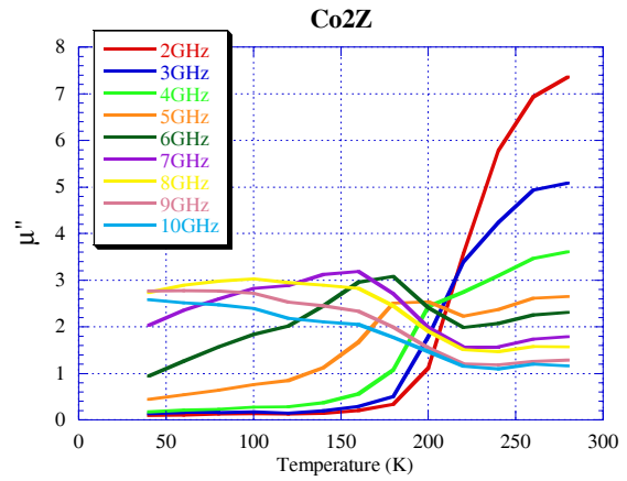
Figure 4: Temperature dependence of imaginary part of Co2Z permeability.
