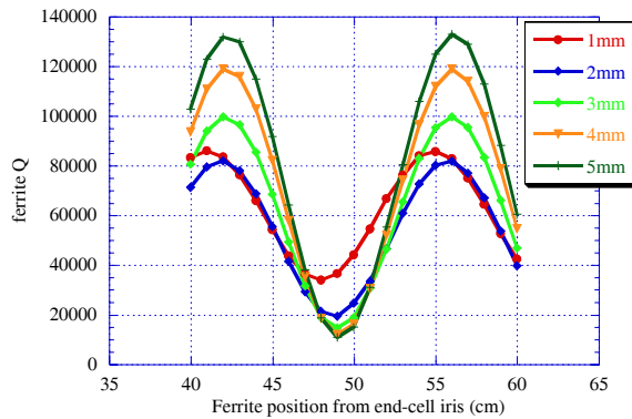
Figure 7: Calculation of ferrite thickness dependence of ferrite Q-value.
