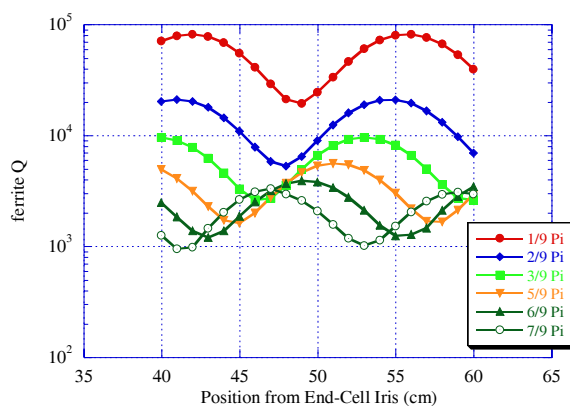
Figure 8: Calculation of TM011-mode dependence of ferrite Q-value.
