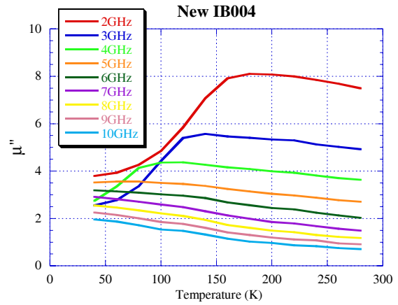
Figure 3: Temperature dependence of imaginary part of new-type IB004 permeability.
