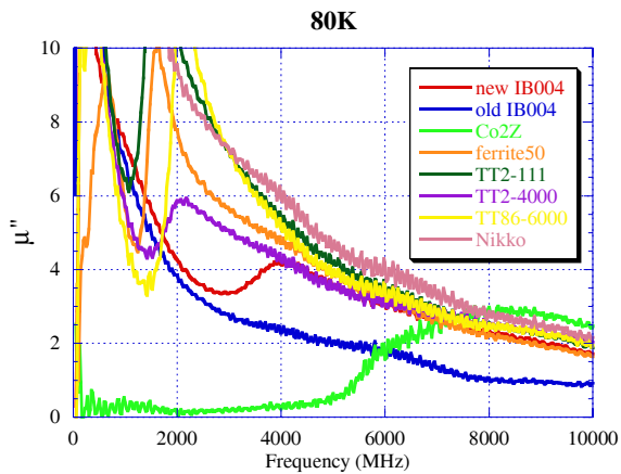
Figure 2: Frequency dependence of ferrite permeability at 80K.
