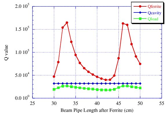
Figure 5: Ferrite, cavity and loaded Q-values as a function of the beam pipe length after ferrite.
