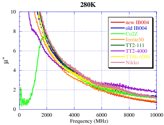
Figure 1: Frequency dependence of ferrite permeability at 280K.
