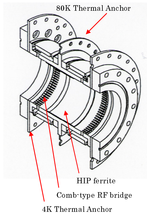
Figure 9: Layout of HOM absorber model
