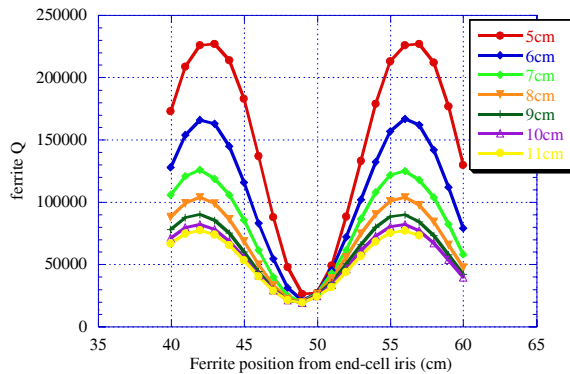
Figure 6: Calculation of ferrite length dependence of ferrite Q-value.
