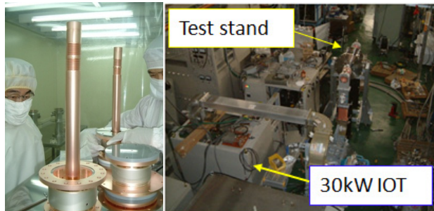
Figure 10 : (Left) proto-type of warm and cold windows. (Right) High power test stand constructed at JAEA.
