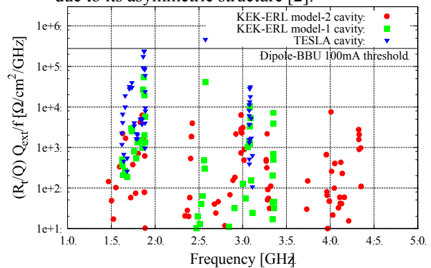
Figure 2 : Spectrum of the dipole HOMs. Details seen in ref [1].
