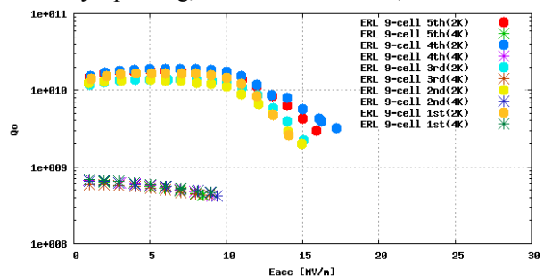
Figure 6 : Results of vertical tests for KEK-ERL model-2 cavity.
