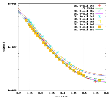
Figure 7 : R_s-1/T curve for KEK-ERL model-2 cavity.
