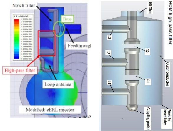
Figure 5: The KEK (left) and BNL (right) HOM antennas for ERL applications.
