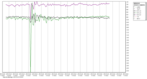
Figure 11: Recorded event during the transport of CMB3. Maximum value of 4.2 g was recorded (green curve).
