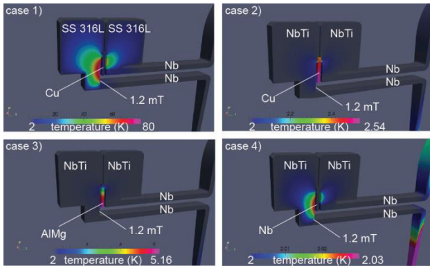
Figure 5: Thermal distributions as in case of Fig. 4, but with a filter line misplaced by +0.5mm from its ideal position. Four cases with material combinations have been studied as indicated.
