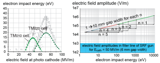
Figure 6: Multipacting assessment for the cavity cells (left) and the filter line (right). See text for more details.
