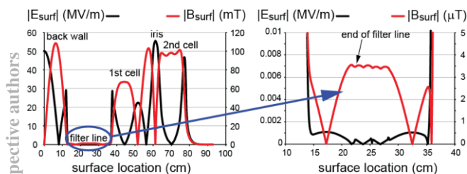
Figure 3: Absolute surface RF electric (black) and magnetic flux density (red), respectively, along the surface interior.
