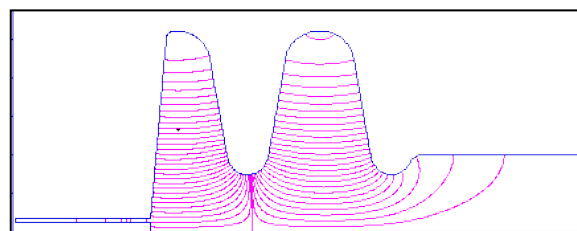
Figure 9: Electric field distribution of superconducting RF electron gun.
