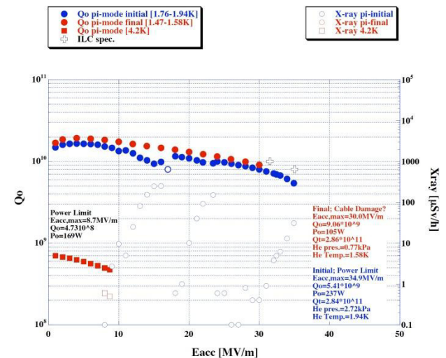
Figure 13: Result of vertical test of cavity that was welded by one batch.
