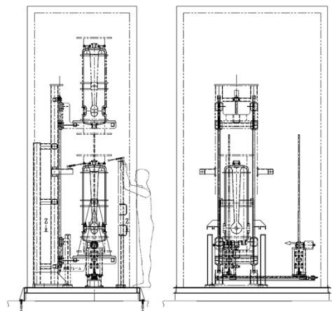
Figure 7: Outline of High pressure rinse facility.
