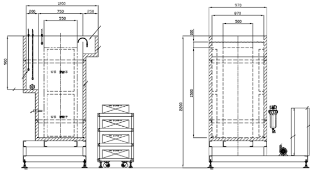
Figure 6: Outline of ultrasonic bath.
