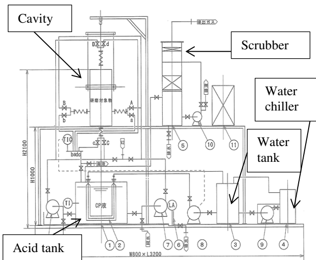
Figure 5: Schematic diagram of BCP facility.
