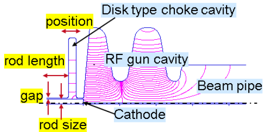
Figure 11: Choke structure of cathode holder.
