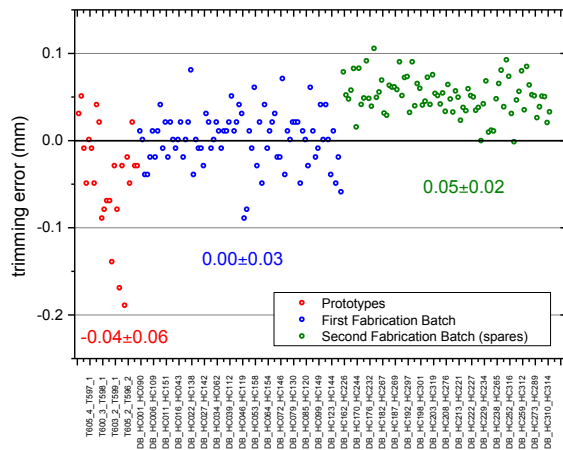
Figure 1: Errors in the implementation of the trimming instructions (i.e. difference between the post/trimming survey with respect to the trimming instruction) in the three production batches. In the label the averages and standard deviations.
