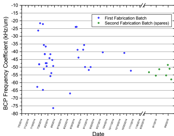
Figure 4: Evolution along time of the frequency response of the cavity to the BCP etching (in units of kHz/um of average material removal). The achievement of a better stability during the first fabrication batch, and especially in the first treatments of the spare series can be appreciated.
