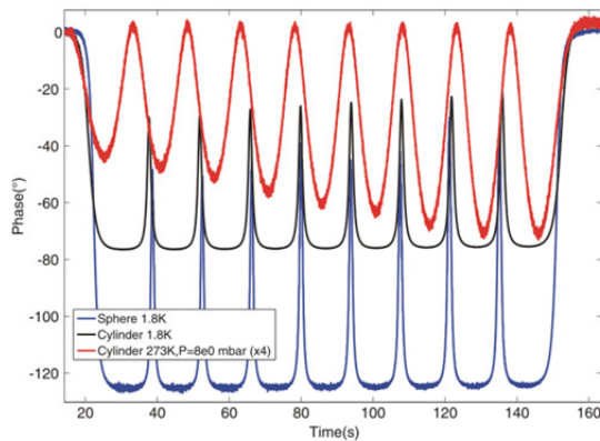
Figure 8: Comparison between warm and cold measurements (spherical/cylindrical) for the fundamental TM_{010} \pi -mode.
