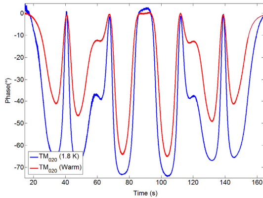
Figure 7: Comparison between warm and cold measurements (cylindrical) for the fundamental TM_{020} 6/9 \pi -mode.
